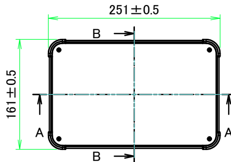
E view
